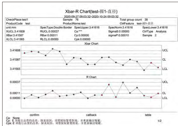
Xbar-R chart
