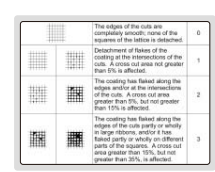
step 3: according to the shedding status, judge the adhesion grade
