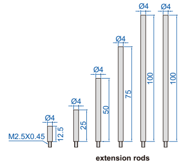
extension rods
