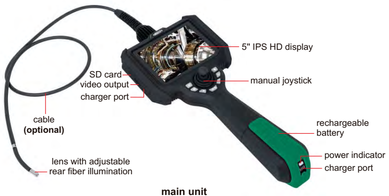
main unit
