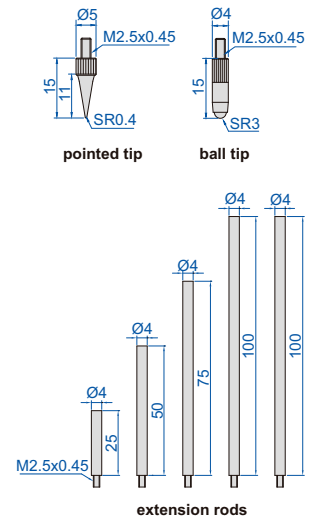
extension rods
