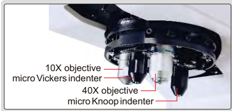
motor driven turret
