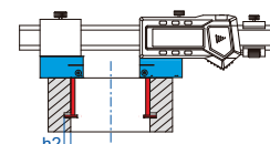
measuring internal groove diameter with spherical measuring face (depth h2 \leq 2.5\text{mm} )
