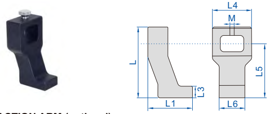
BEVEL REACTION ARM (optional)
