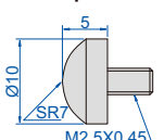
spherical point
