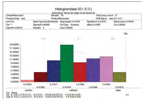
Histogram
