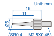
needle point
