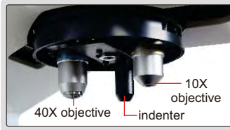
motor driven turret
