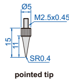
pointed tip
